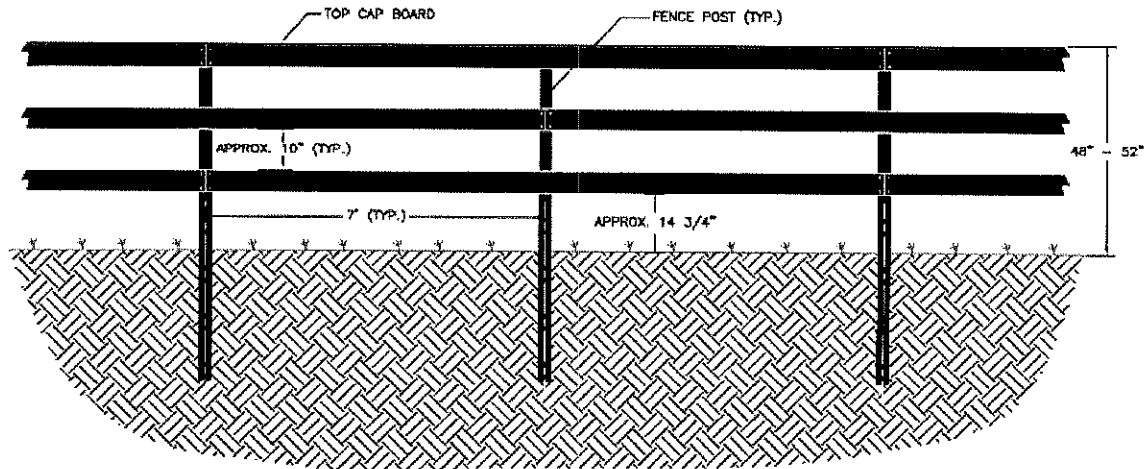
FENCING DETAIL
